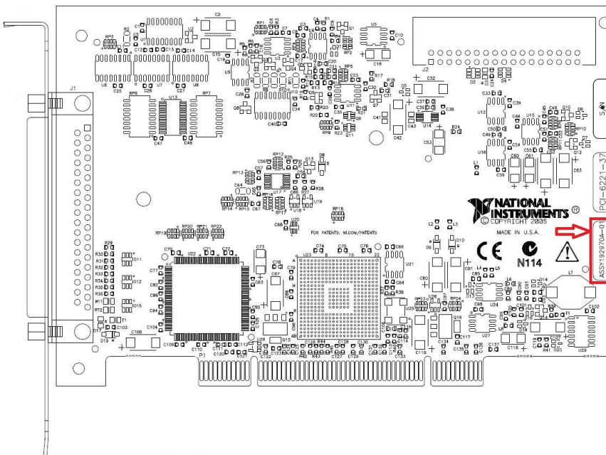
PCI-6221 (37-PIN) – Primary Side
