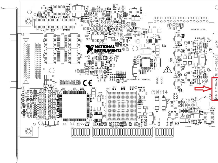
PCI-6220/21/24/29 – Primary Side
