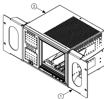
Figure 3. NI Chassis Rack Mount Kit Components
