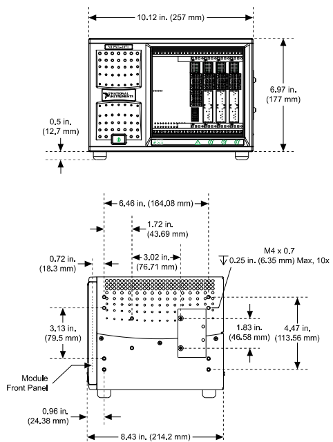
Figure 2. PXle-1071 Chassis Dimensions (Bottom)
