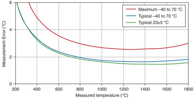
Figure 8. NI 9210 with Spring Terminal Thermocouple Type B Errors
