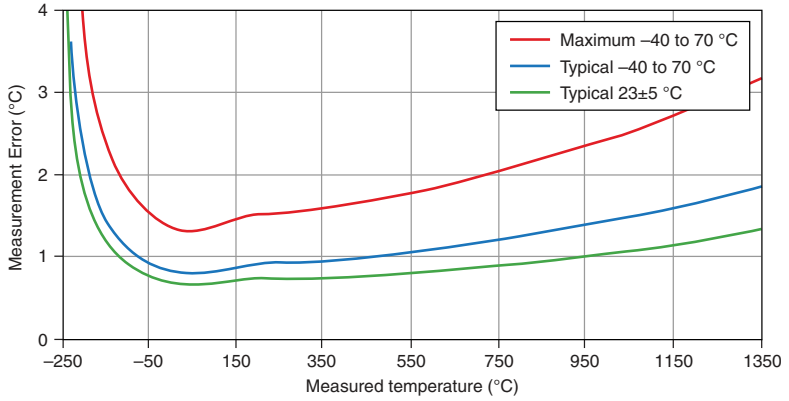
Figure 4. NI 9210 with Spring Terminal Thermocouple Type K Errors
