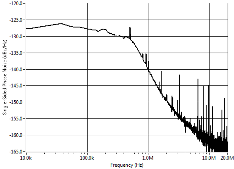
Figure 11. Phase Noise with 800 MHz Input Tone, Measured
