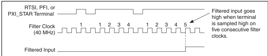
Figure 9-3. Filter Example
