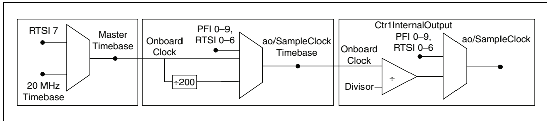
Figure 5-5. Analog Output Engine Routing Options
