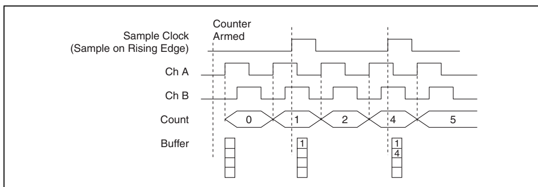
Figure 7-19. Buffered Position Measurement
