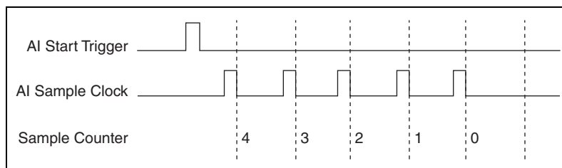
Figure 4-7. Typical Posttriggered DAQ Sequence
