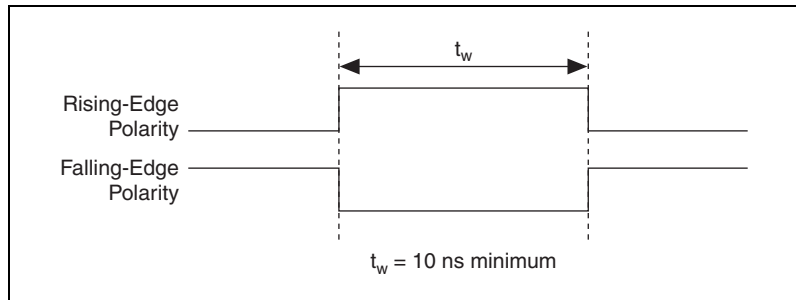
Figure 5-9. AO Start Trigger Timing Requirements
