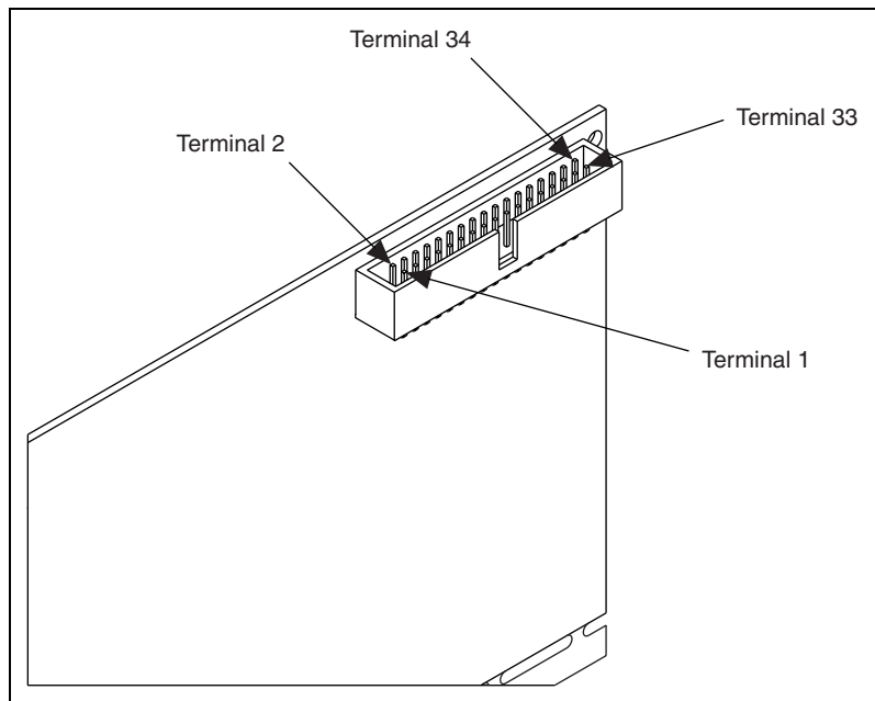
Figure 10-2. NI 6236 RTSI Pinout
