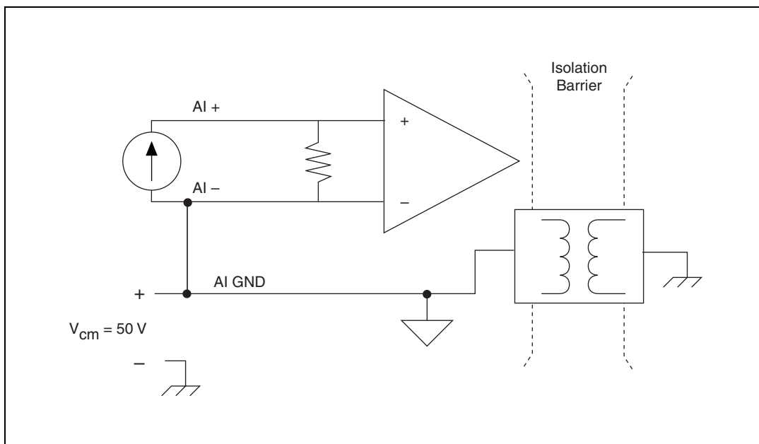
Figure 4-4. Current Measurement at High Voltage Levels
