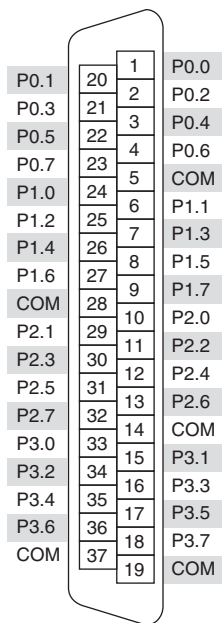
Figure 3-1. NI 6510 Pin Assignments
