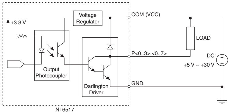
Figure 4-13. NI 6517 Output Signal Connection Example
