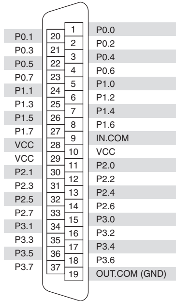
Figure 3-14. NI 6518 Pin Assignments
