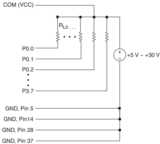
Figure 4-16. NI 6519 GND Connection Example
