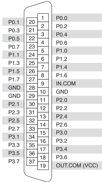
Figure 3-15. NI 6519 Pin Assignments
