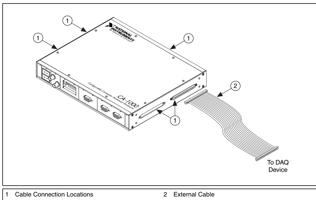
Figure 12. Installing External Cable Assemblies
