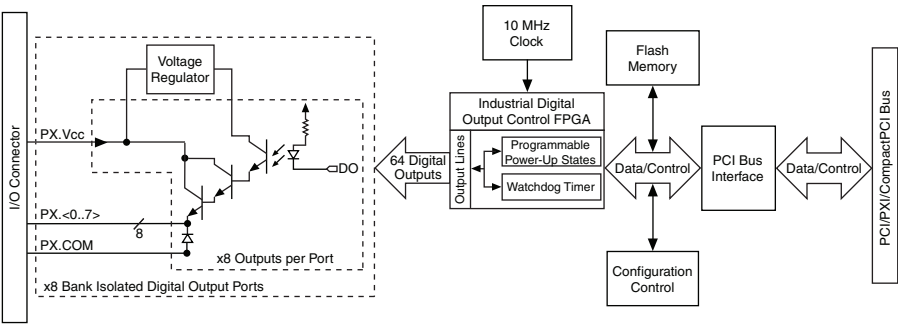
Figure 1-4. NI 6513 Block Diagram
