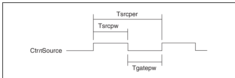
Figure 3-9. Timing Requirements for CtrnSource Signal
