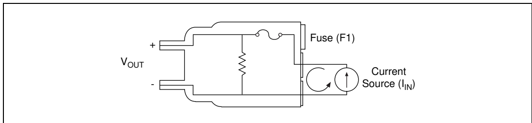
Figure 2. CSM Internal Construction
