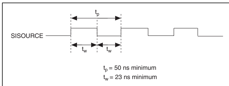
Figure 3-20. SISOURCE Signal Timing
