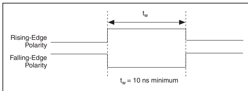
Figure 3-18. CONVERT* Input Signal Timing
