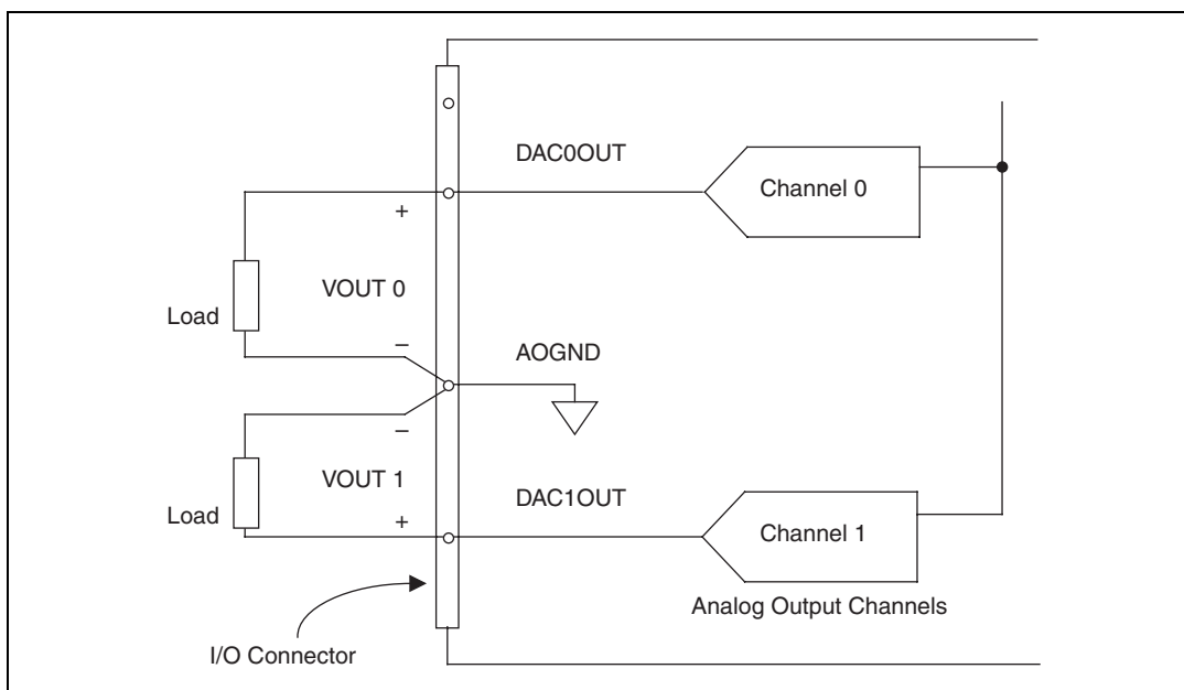
Figure 3-9. AO Connections
