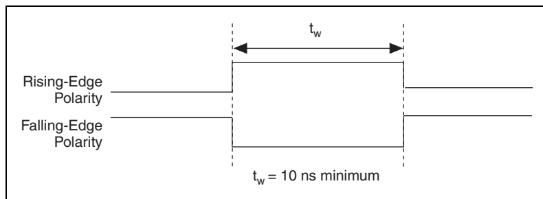
Figure 3-23. WFTRIG Input Signal Timing
