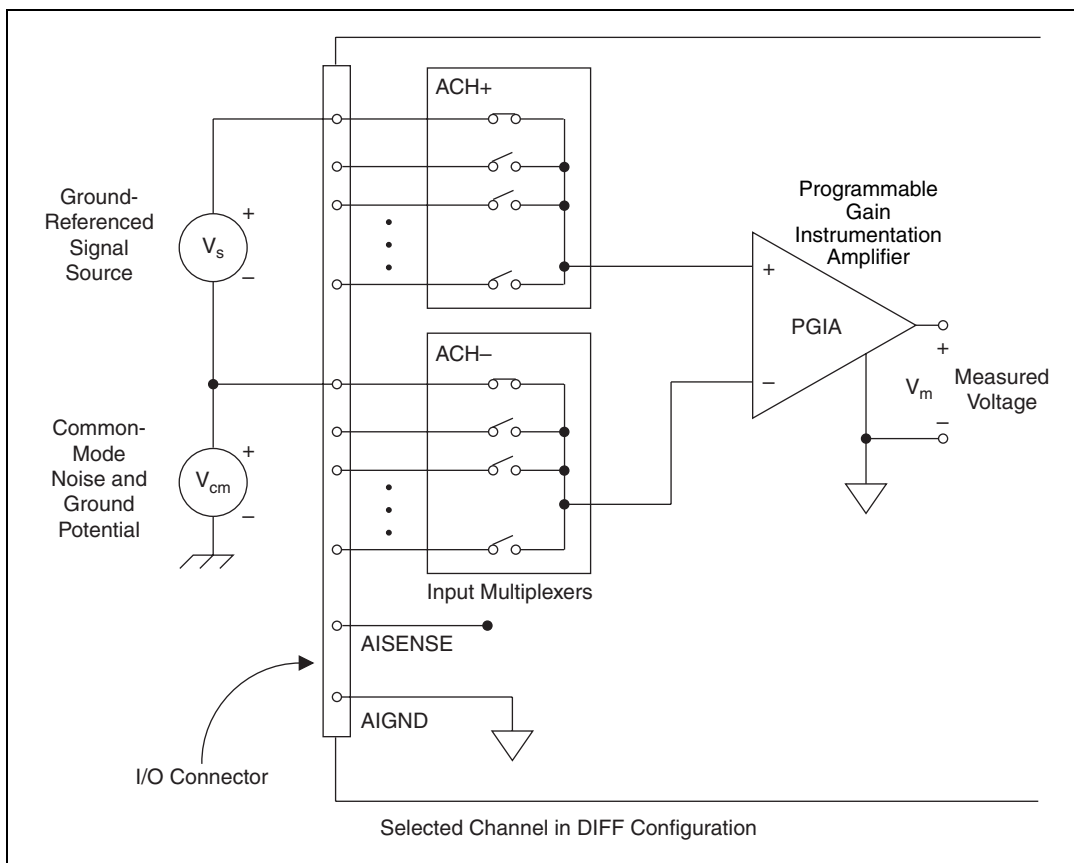
Figure 3-4. Differential Input Connections for Ground-Referenced Signals
