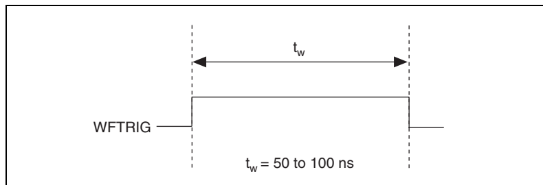
Figure 3-24. WFTRIG Output Signal Timing
