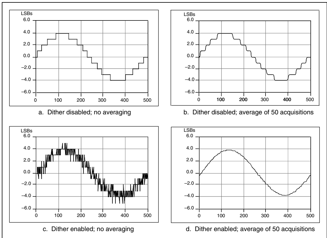
Figure 2-2. Dither
