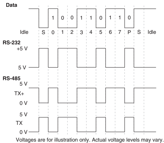
Figure 13. UART Data Frame Example
