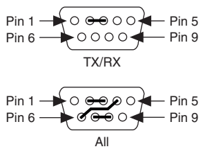
Figure 7. RS-232 Loopback
