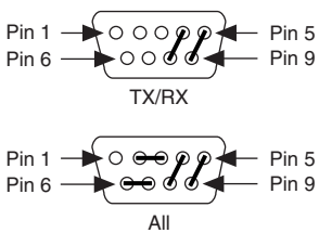
Figure 9. RS-485/422 Loopback
