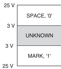
Figure 8. RS-232 Signals
