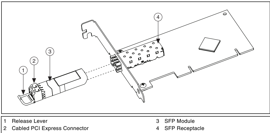
Figure D-1. SFP Module Removal
