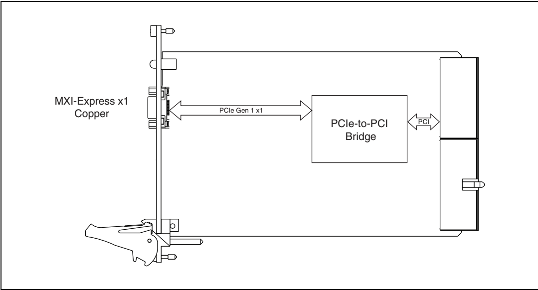
Figure C-2. NI PXI-8361 (199991x-01L) Block Diagram
