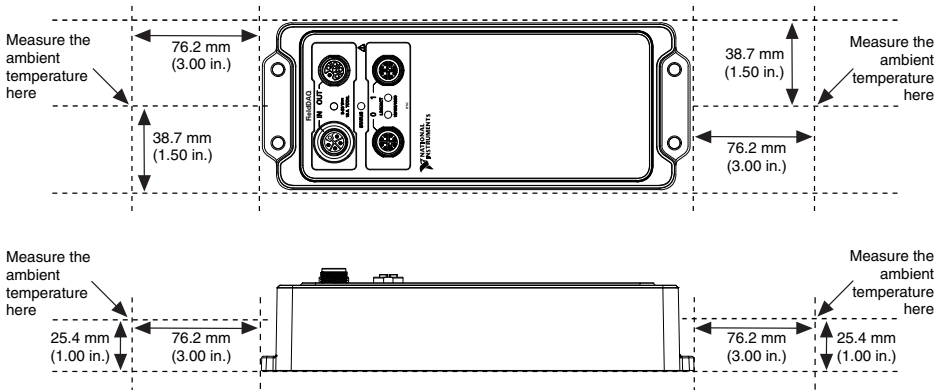
Figure 24. Ambient Temperature Locations, Horizontal Mounting Configuration
