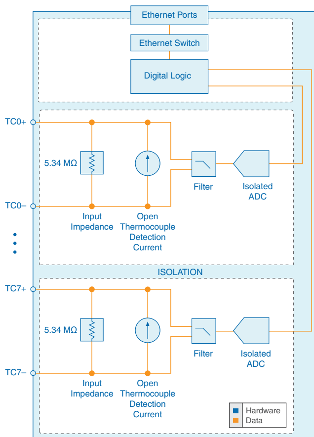
Figure 8. FD-11613 Block Diagram
