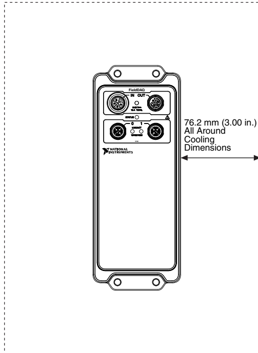
Figure 22. Cooling Dimensions
