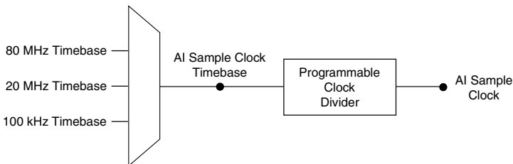
Figure 11. AI Sample Clock Timing Options
