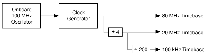
Figure 13. Clock Routing Circuitry
