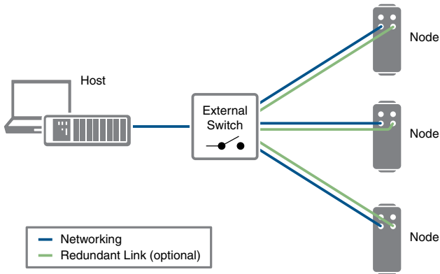
Figure 17. Star Topology
