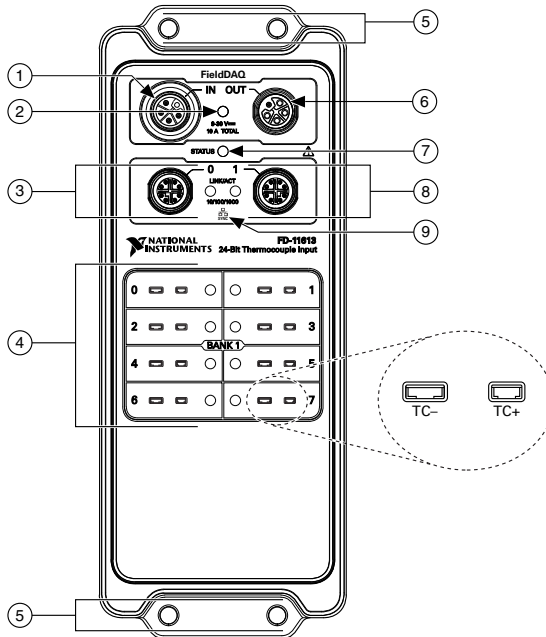
Figure 1. FD-11613 Front Panel
