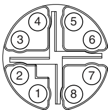
Figure 14. Ethernet Connector Pinout
