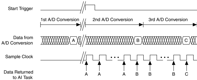
Figure 12. Sample Clock Timing Example
