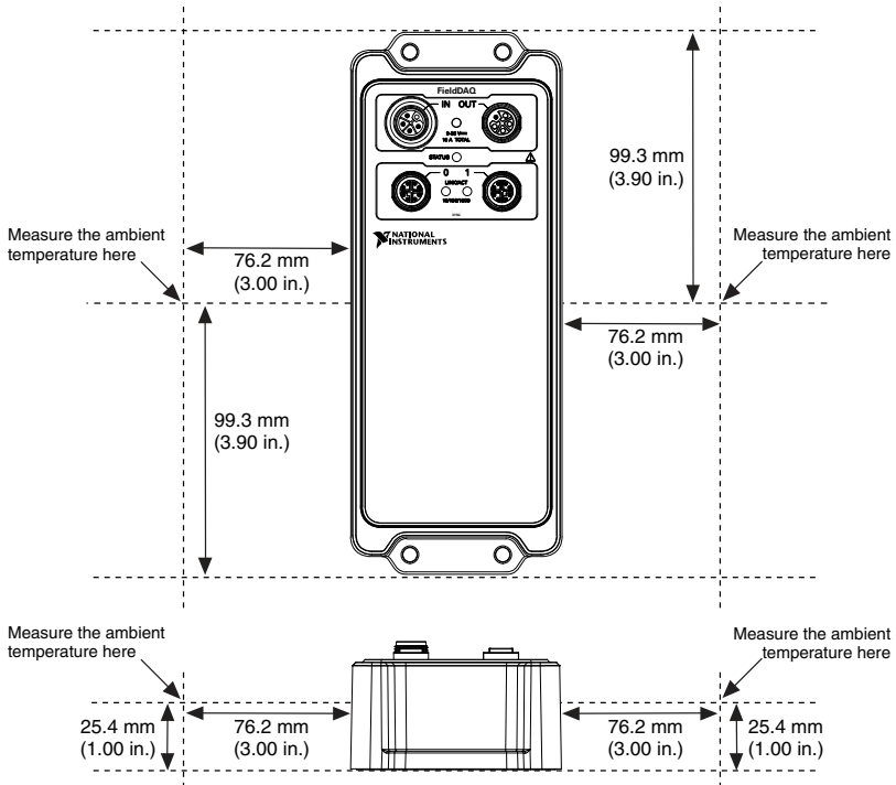
Figure 25. Ambient Temperature Locations, Vertical Mounting Configuration
