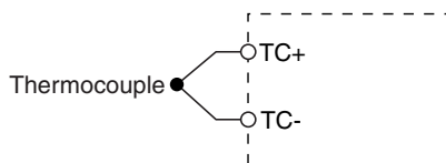
Figure 10. Connection Diagram
