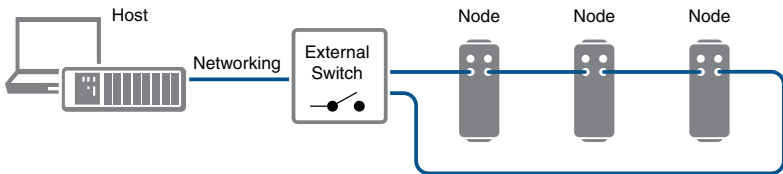
Figure 16. Ring Topology
