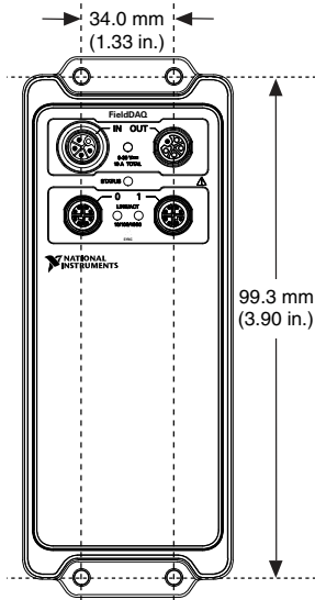
Figure 26. Surface Mounting Dimensions
