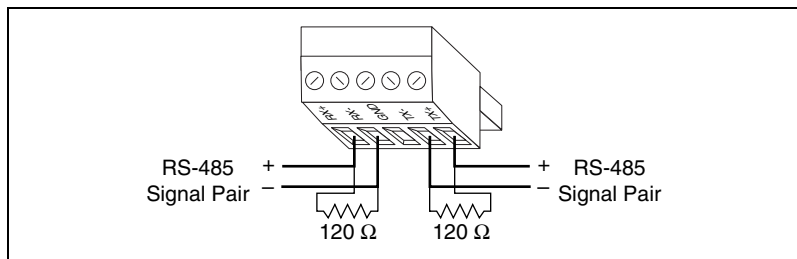
Figure 2-12. Terminating RS-485 Using the Combicon Adapter
