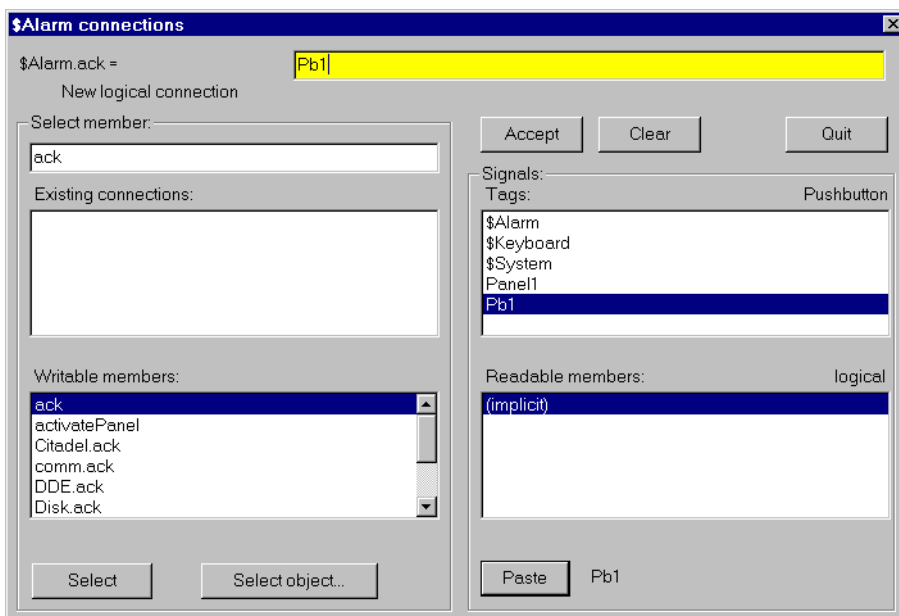
Figure 18-9. Edit Connections Dialog Box for using $Alarm
