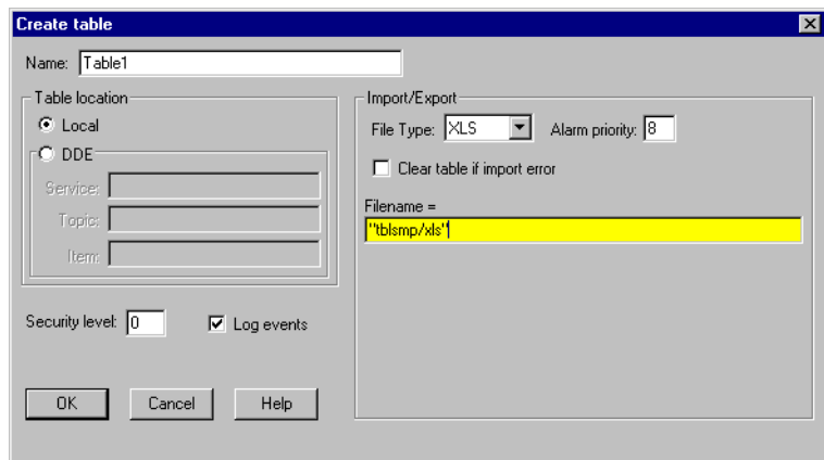
Figure 2-10. DataTable Definition Parameters Dialog Box
