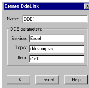
Figure 2-17. DdeLink Definition Parameters Dialog Box (Same Computer)
