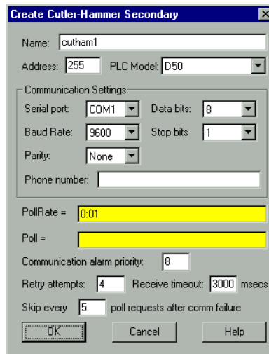
Figure 3-10. Cutler-Hammer Definition Parameters Dialog Box
