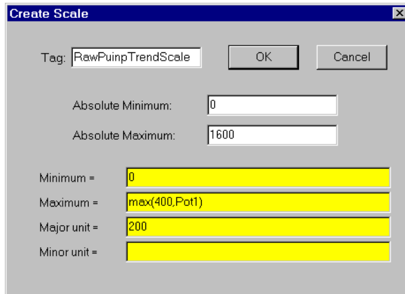
Figure 18-109. Scale Definition Parameters Dialog Box
