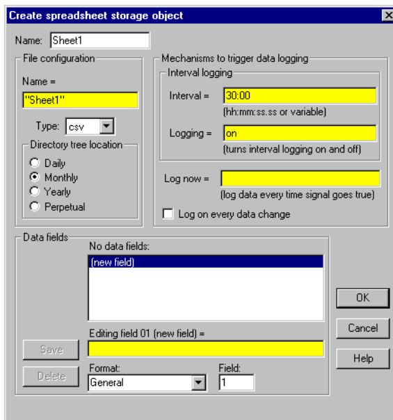
Figure 2-90. Spreadsheet Configuration Parameters Dialog Box
