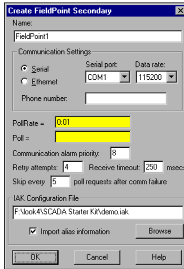
Figure 16. Create FieldPoint Secondary Dialog Box
