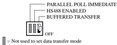
Figure 9. DIP Switch Setting for Buffered Mode
