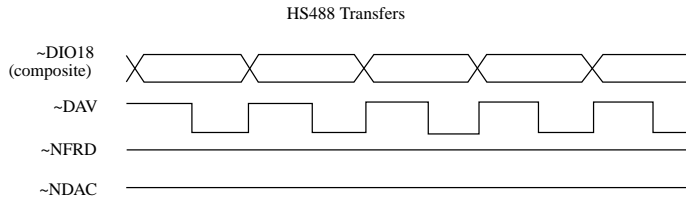
Figure 16. HS488 Transfers
