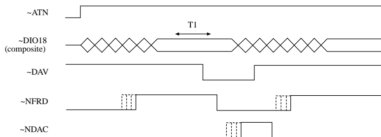
Figure 19. Listener Is HS488-Capable
