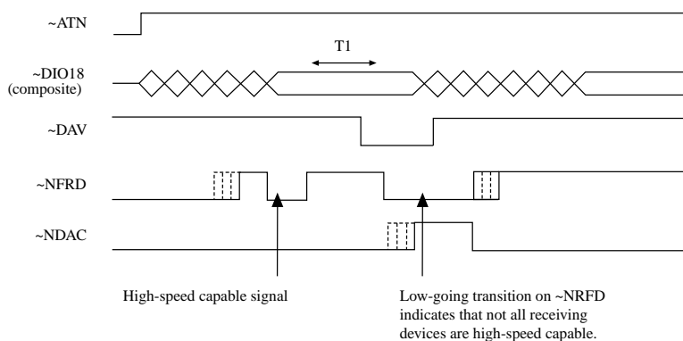
Figure 18. HS488-Capable Talker
