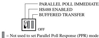
Figure 11. DIP Switch Setting for Immediate PPR Mode
