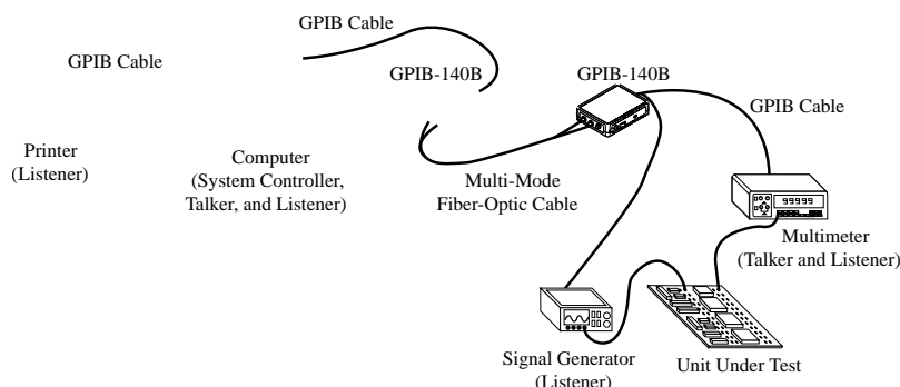
Figure 1. Typical Extension System (Physical Configuration)
