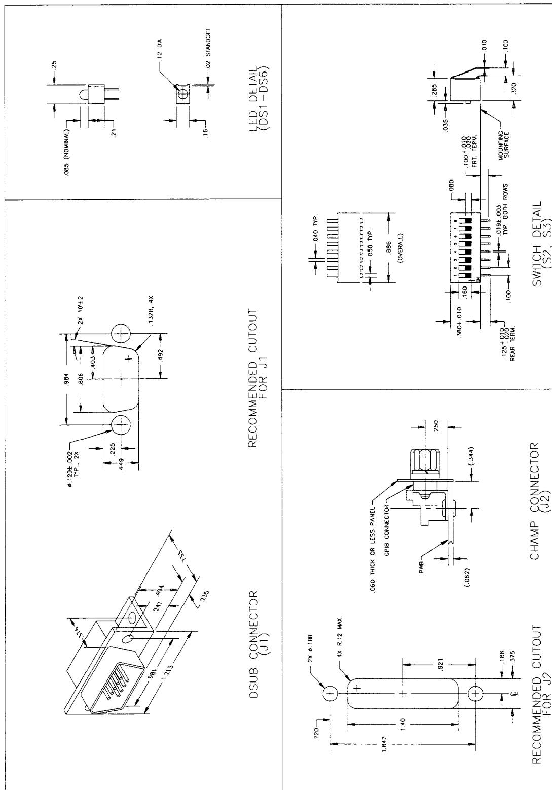
Figure 4. Measurements for Mounting Connectors, Switches, and LEDs
