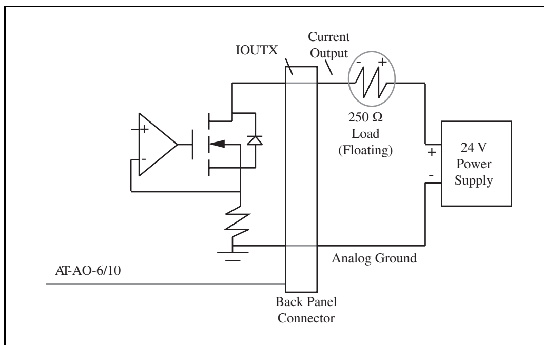
Figure 3-5. Possible Current Loop Connection
