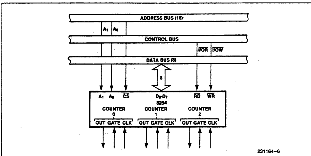
Figure 6. 8254 System Interface
