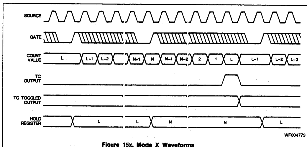
Figure 15x. Mode X Waveforms
