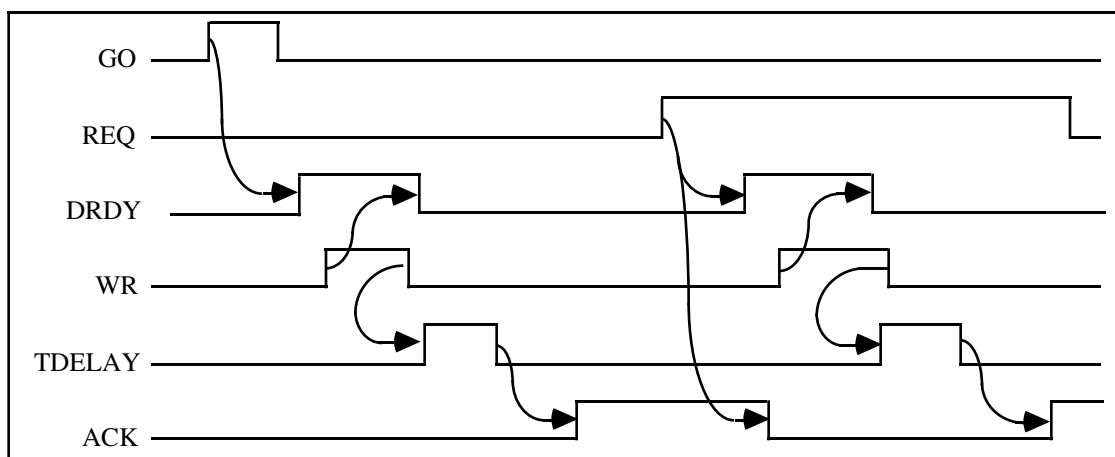
Figure 4-1. Level Mode Write Handshake Timing
