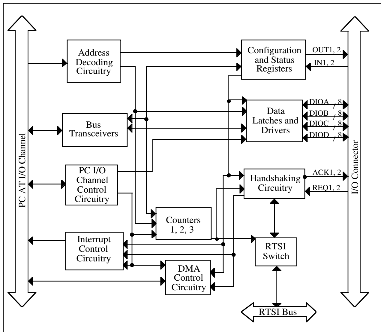
Figure 3-1. AT-DIO-32F Block Diagram
