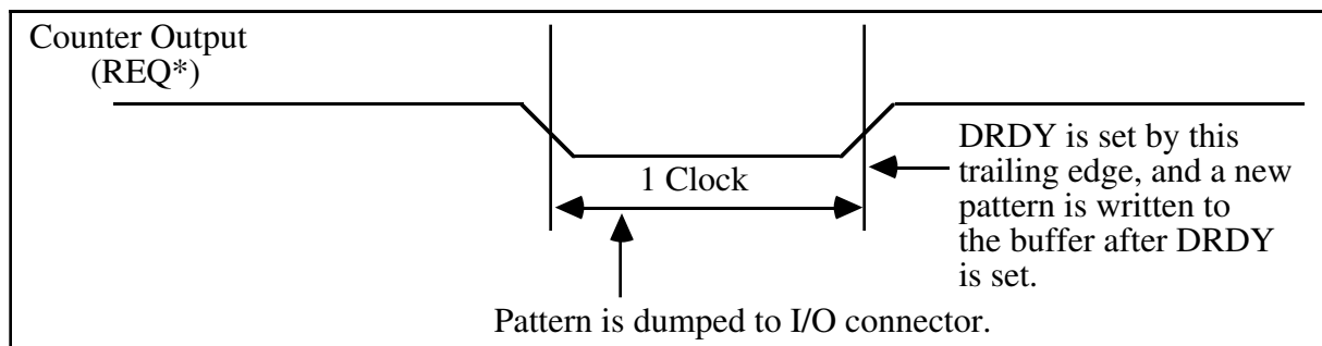
Figure 4-8. Pattern Generation
