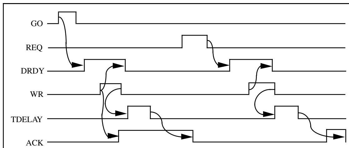
Figure 4-6. Trailing Edge Mode Write Handshake Timing
