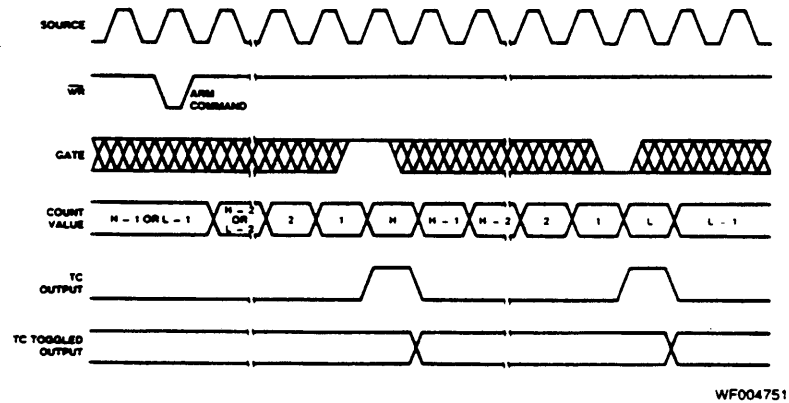
Figure 15s. Mode S Waveforms
