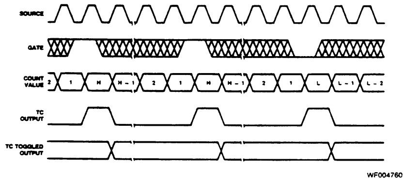
Figure 15v. Mode V Waveforms
