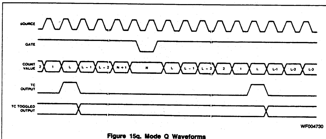
Figure 15q. Mode Q Waveforms
