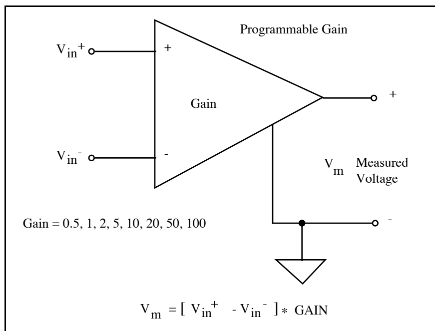
Figure 2-6. AT-MIO-64F-5 PGIA
