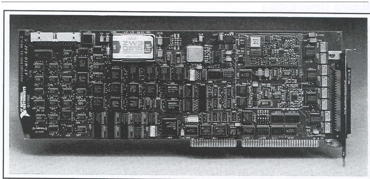
Figure 1-1. AT-MIO-64F-5 Board
