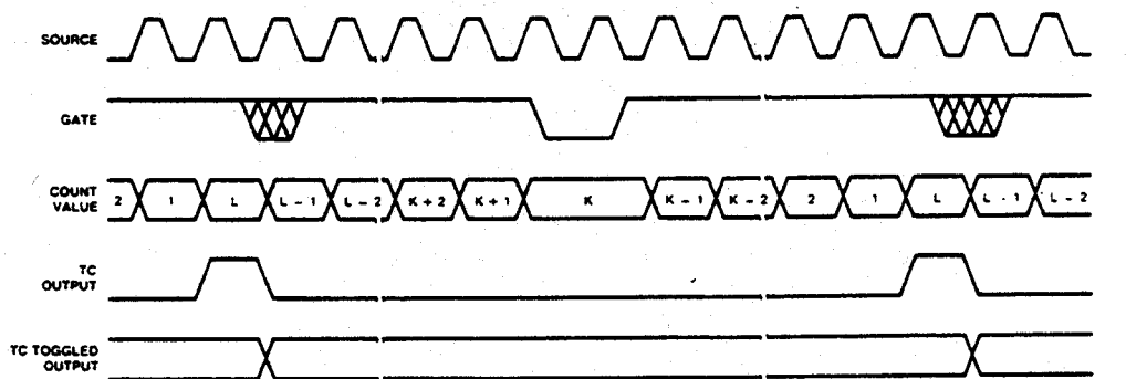
Figure 15e. Mode E Waveforms
