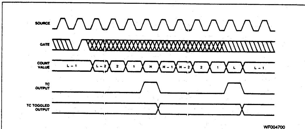
Figure 15l. Mode L Waveforms
