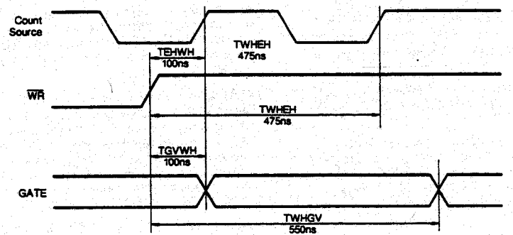
Figure A3. TEHWH/TGVWH Timing Diagram
