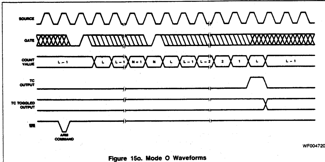
Figure 15o. Mode O Waveforms
