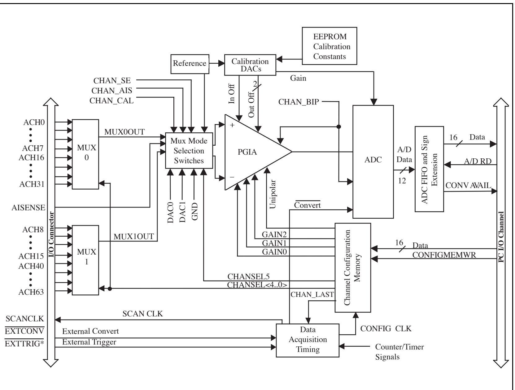
Figure 3-3. Analog Input and Data Acquisition Circuitry Block Diagram
