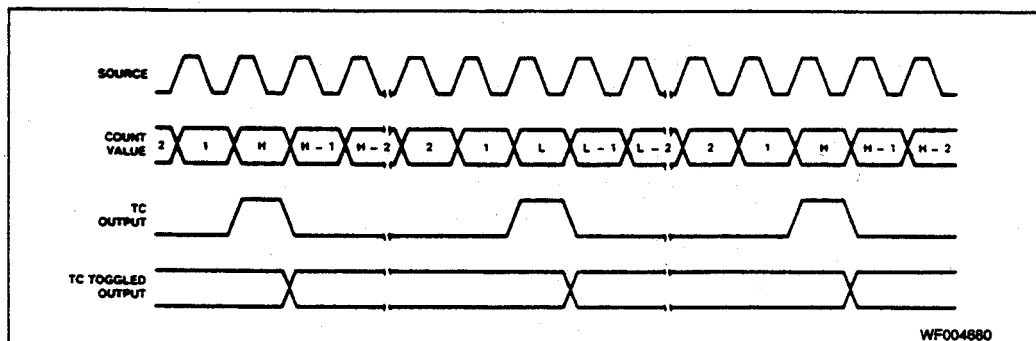
Figure 15j. Mode J Waveforms
