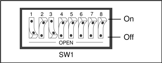
Figure A-2. SW1 Default Mode Switch Settings
