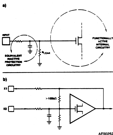
Figure 3. Input Circuitry
