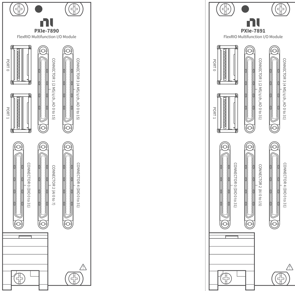
Figure 1. PXIe-7890 and 7891 Front Panels
