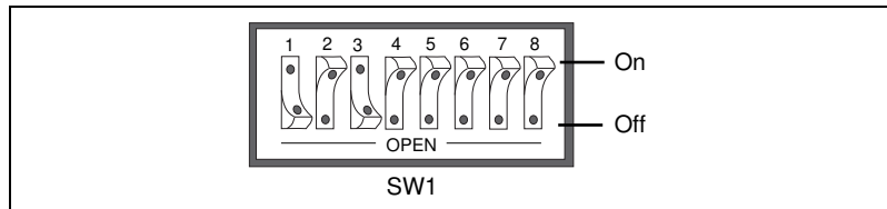
Figure 3-2. SW1 Default Mode Switch Settings
