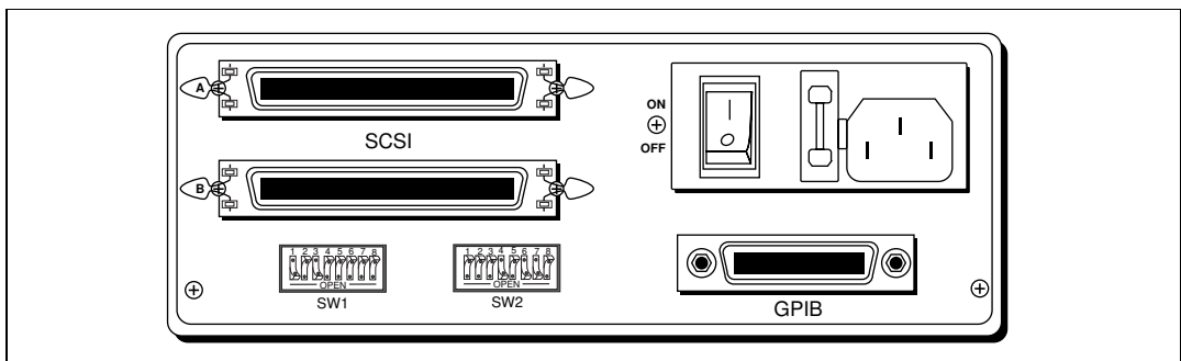
Figure 3-1. GPIB-SCSI-A Rear Panel
