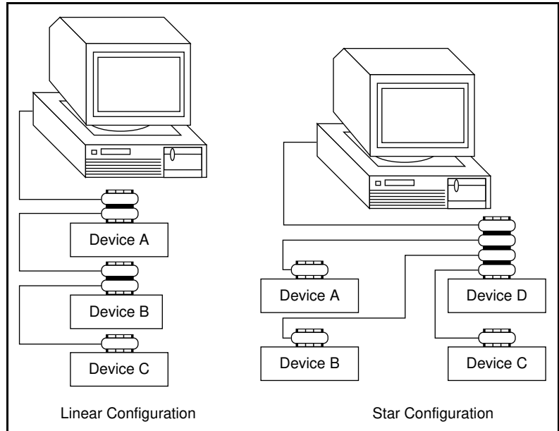
Figure 1-1. Linear and Star System Configuration
