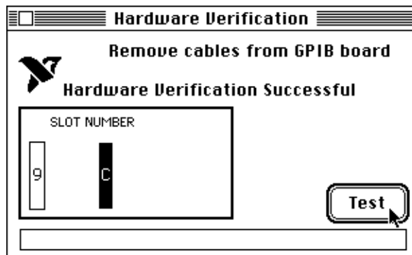
Figure 4-3. Hardware Verification Window after Successful Completion of Tests
