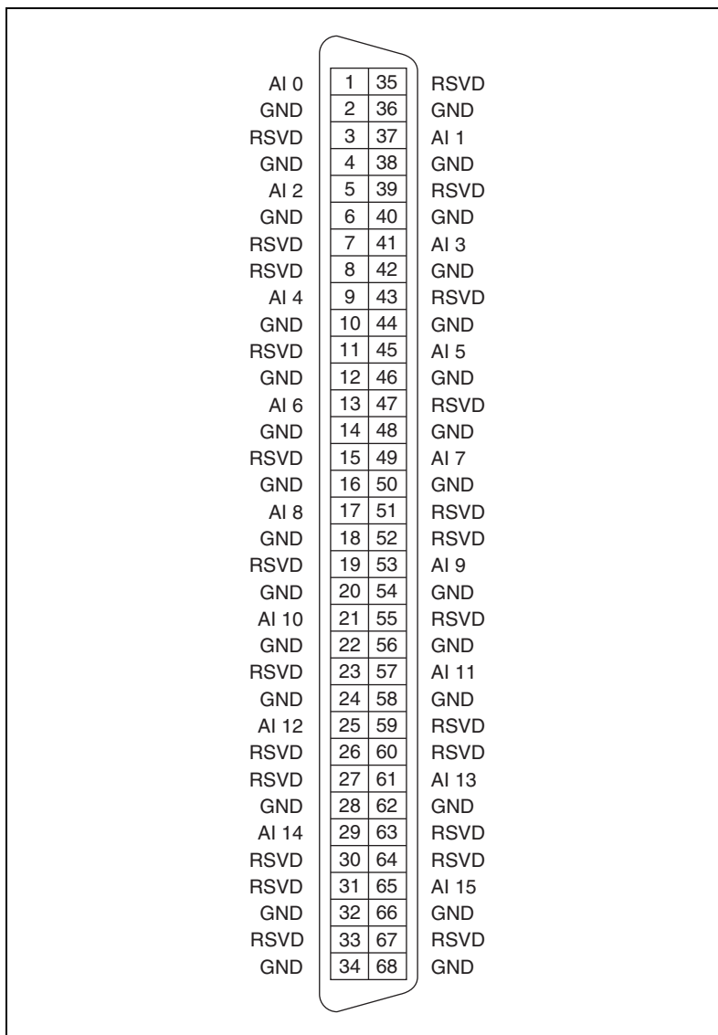
Figure 9. NI SMB-2147 VHDCI Connector Pinout
