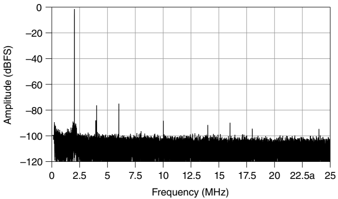
Figure 3. Characteristic Dynamic Performance, Spectrum-64,000 Samples, Coarse Gain 12 dB, 2 MHz, -1 dBFS Differential-Ended Input Signal
