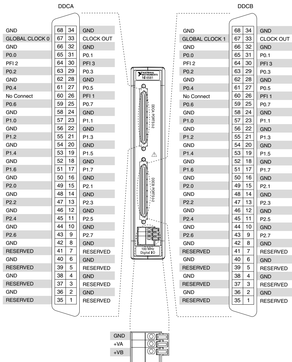
Figure 2. NI 6581/6581B Connector Pin Assignments
