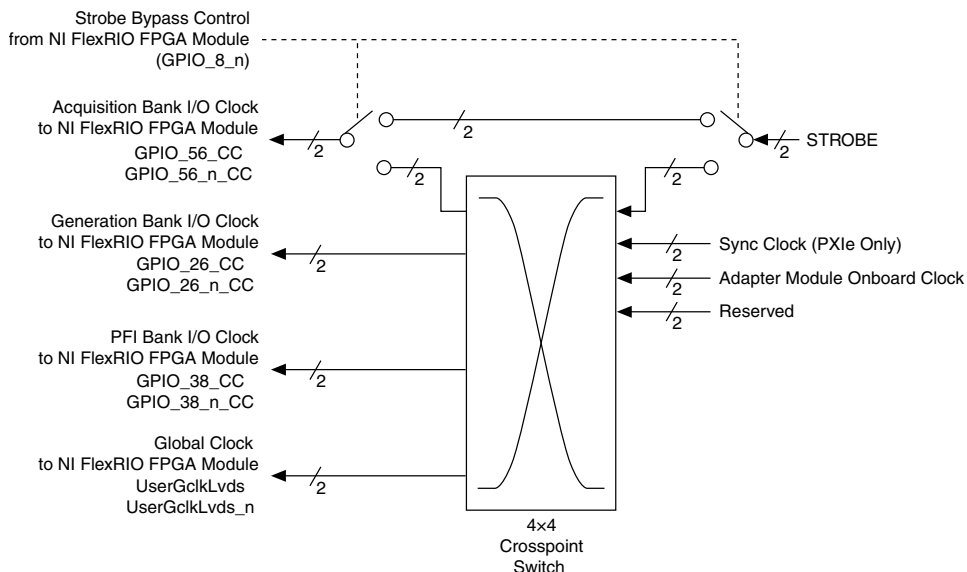
Figure 9. Crosspoint Switch
