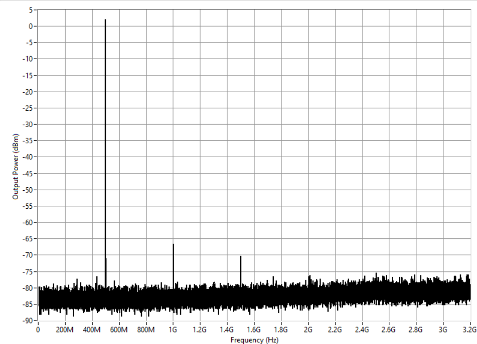
Figure 8. Single Tone Spectrum (Dual Channel Mode, 501 MHz 0 dBFS), Measured 17
