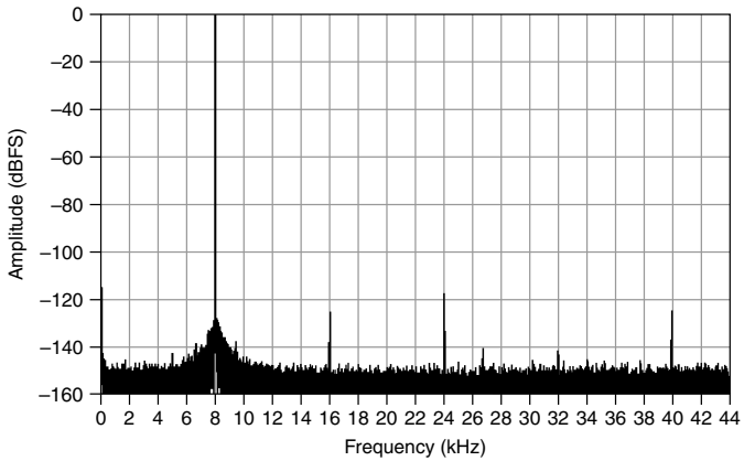
Figure 6. FFT of -1 dBFS, 8 kHz Tone Sampled at 102.4 kS/s (Unaveraged Computation of 262,144 Samples)
