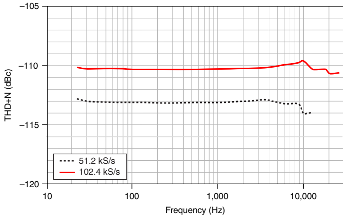
Figure 8. THD+N versus Frequency
