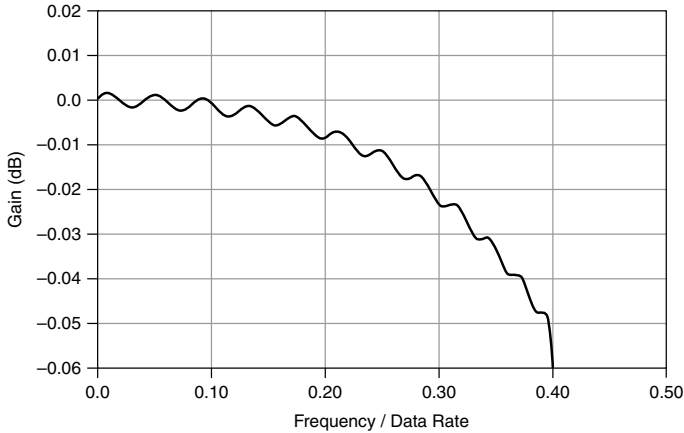
Figure 2. Typical Passband Flatness in DC Coupling for the NI 9251 with mini XLR at the Maximum Data Rate
