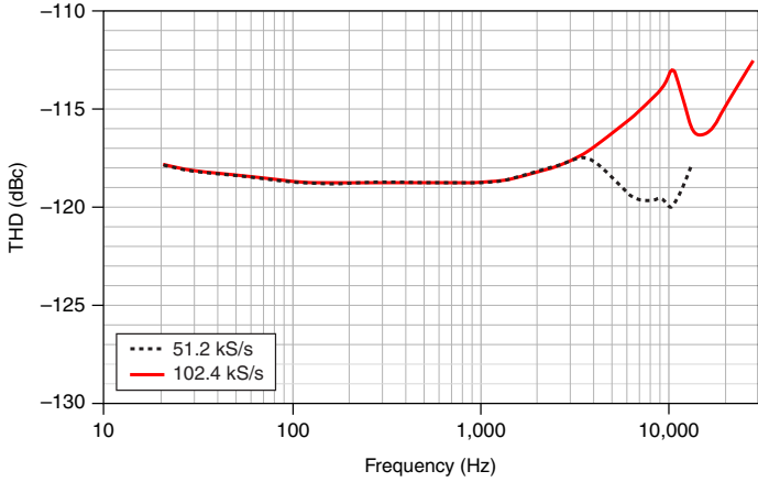
Figure 7. THD versus Frequency
