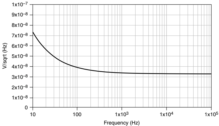
Figure 4. Spectral Noise Density versus Frequency
