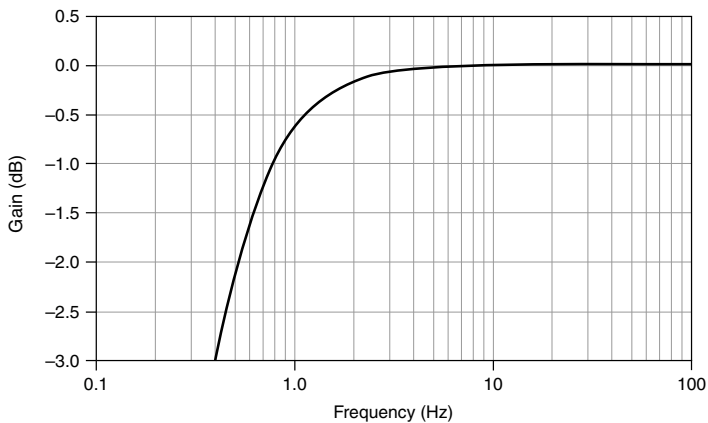
Figure 3. High Pass Filter Frequency Response
