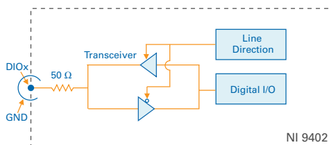
Figure 1. NI 9402 Circuitry for One Channel
