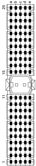
Figure 1. XJ2 Connector Pinout
