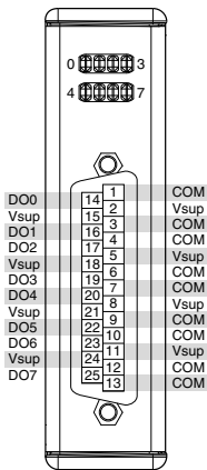
Figure 1. NI 9475 Pinout
