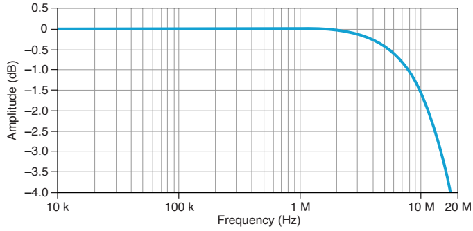
Figure 1. Frequency Response in High-Speed Mode with Analog Filter Enabled
