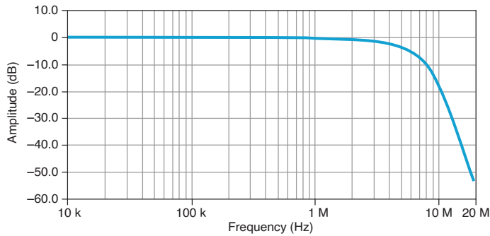
Figure 1. Frequency Response in High-Resolution Mode
