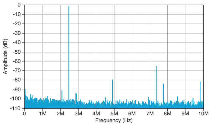
Figure 1. Single-Tone Spectrum at (-1 dB FS, 2.45 MHz)
