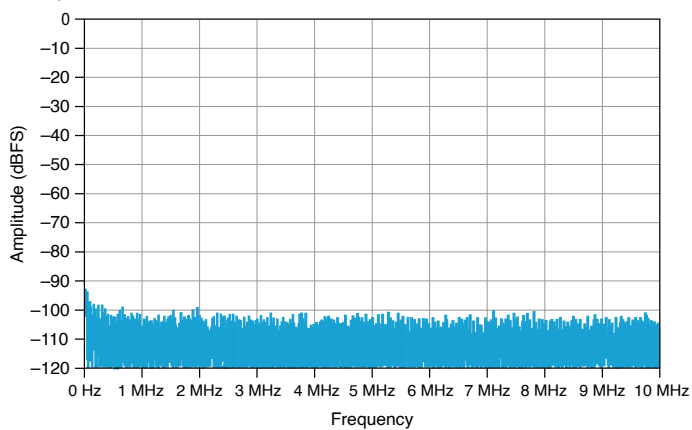
Figure 1. Idle Channel FFT in High-Speed Mode with Analog Filter Disabled (20 MS/s, 32,768 point FFT)
