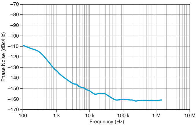
Figure 1. Phase Noise
