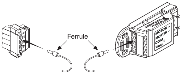
Figure 6. 4-Terminal Screw Terminal Connector or Accessory with a Ferrule
