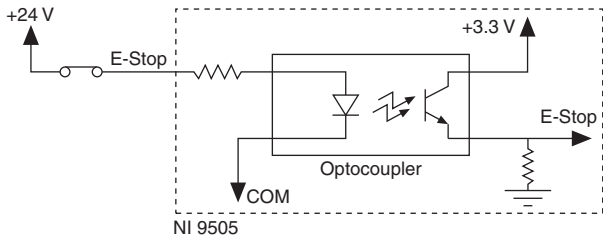
Figure 10. Emergency Stop Input Circuit
