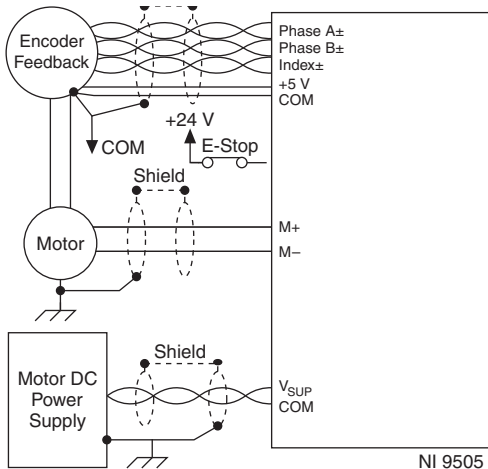
Figure 4. NI 9505 Connections
