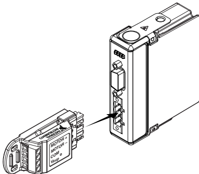
Figure 5. NI 9505 Module with Optional Screw Terminal Accessory
