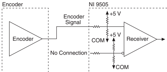
Figure 9. Single-Ended Encoder Input Circuit
