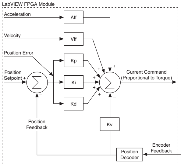
Figure 2. LabVIEW FPGA Module NI 9505 PID Loop
