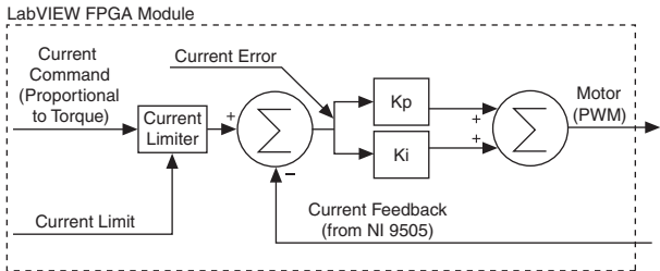
Figure 3. LabVIEW FPGA Module NI 9505 Current Loop
