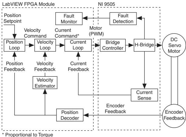
Figure 1. NI 9505 Block Diagram
