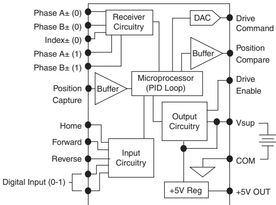
Figure 4. NI 9516 Block Diagram
