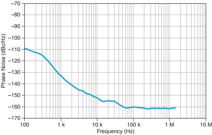
Figure 9. Phase Noise
