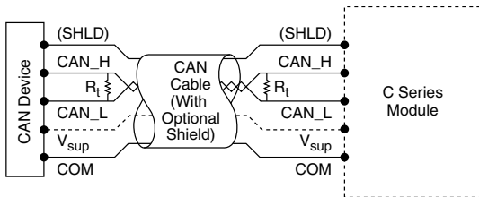
Figure 2. Connecting the NI 9862 to a CAN Device
